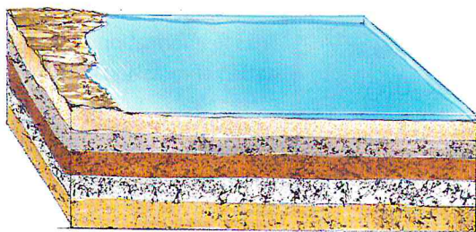
Figure 13 An angular unconformity results when horizontal layers cover tilted, eroded layers.
