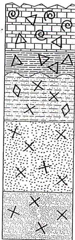
Outcrop 2
