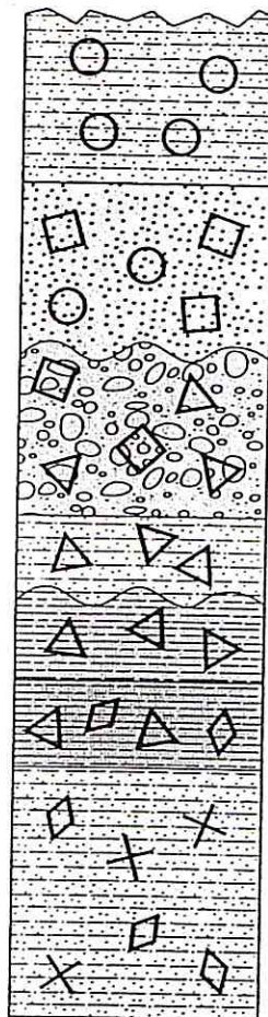
Outcrop 3
