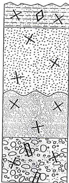
Outcrop 1
