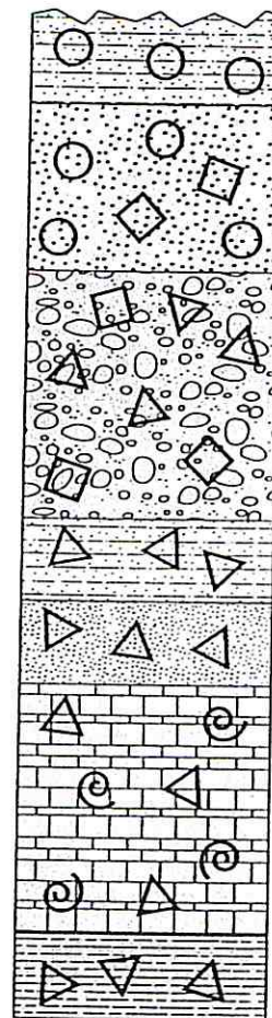
Outcrop 4
