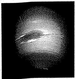
Neptune
