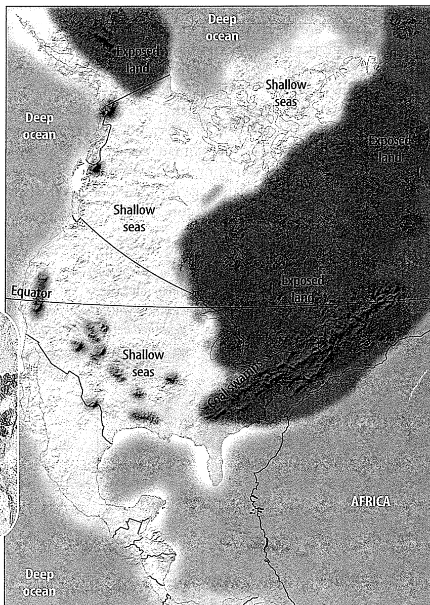
Figure 9 The equator passed through North America 310 million years ago. At this time, warm, shallow seas and coal swamps covered much of the continent, and ferns like the Neuropteris , below, were common.
