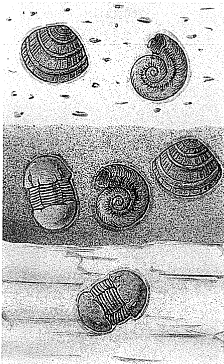
Figure 8 The fossils in a sequence of sedimentary rock can be used to estimate the ages of each layer. The chart shows when each organism inhabited Earth.
