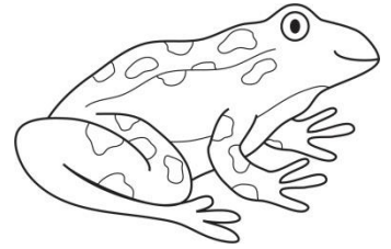
frog
