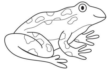
frog
