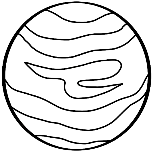
Neptune
