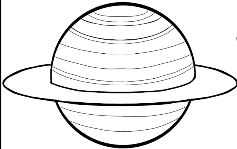
Saturn
