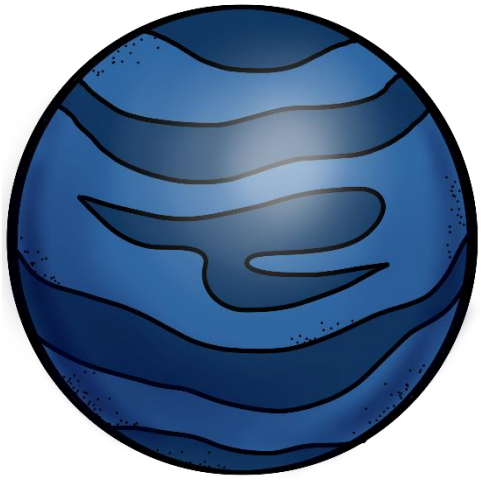
Neptune
